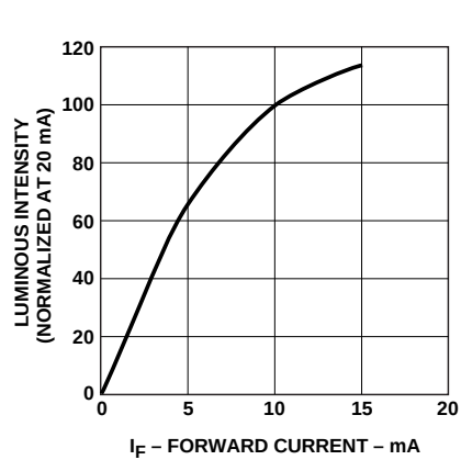
Figure 3. Luminous intensity vs. forward current.
